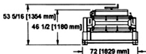
SINGLE TANDEM-SCREEN SHAKER WEIGHT: 2500 LBS. (1136 KG.)
