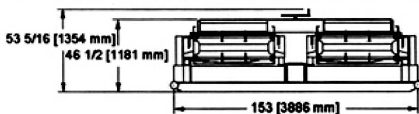
DUAL TANDEM-SCREEN SHAKER WEIGHT: 5000 LBS. (2773 KG.)
