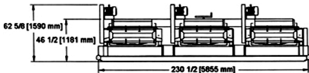
TRIPLE TANDEM-SCREEN SHAKER WEIGHT: 7800 LBS. (3545 KG.)
